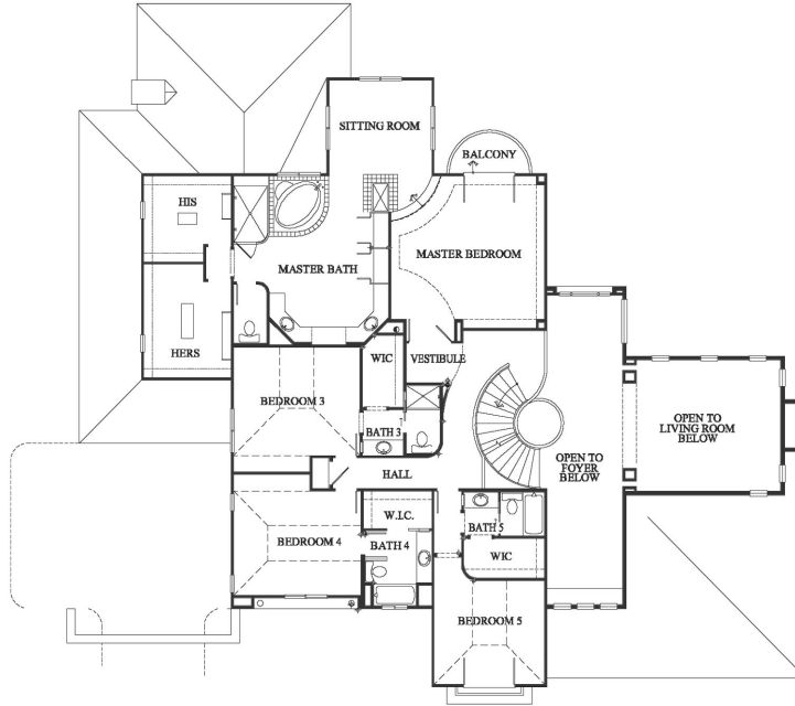
UPPER FLOOR
